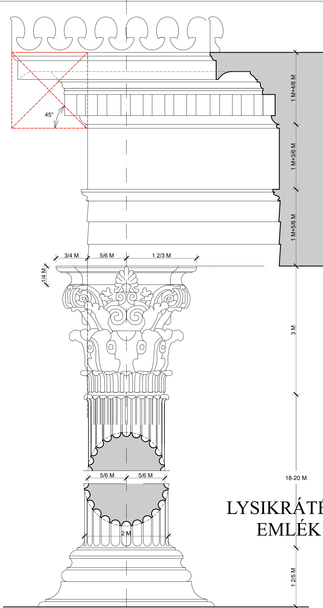
GREEK CORINTHIAN ORDER - LYSICRATES MEMORIAL
